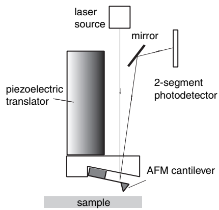
FIGURE 1. Schematic of AFM (see text for details).
