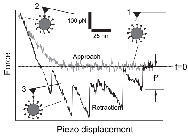
FIGURE 3. Force versus displacement curves of the interaction between a streptavidin-functionalized tip and a biotinylated agarose bead. The measurement recorded the force on the AFM cantilever on approach and retraction of the cantilever from the agarose bead. The inserts illustrate the deflection of the cantilever at different points during the measurement. f^* is the rupture force.
